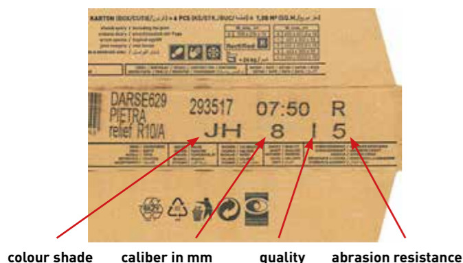
Fig.1 Cardboard packaging for glazed tiles
